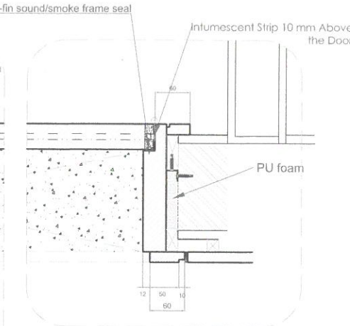
D4 Typical Frame detail
